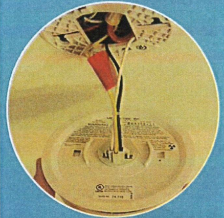
HARD- WIRED CARBON MONOXIDE ALARM
