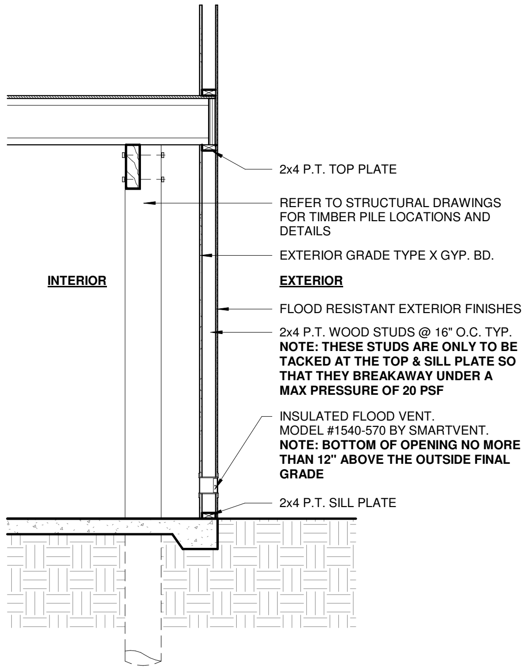
1 TYPICAL BREAKAWAY WALL 1/2" = 1'-0"
